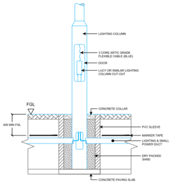
TYPICAL DUCTED LIGHTING COLUMN DETAIL SCALE:NTS
