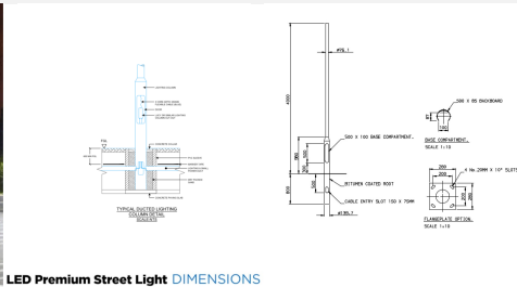
LED Premium Street Light DIMENSIONS
