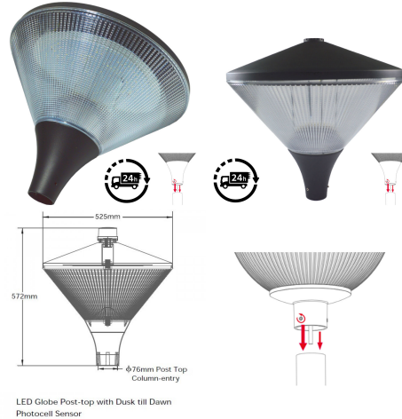
LED Globe Post-top with Dusk till Dawn Photocell Sensor
